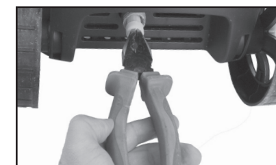
Pulling the filter out of the water inlet fitting, Fig. 14
